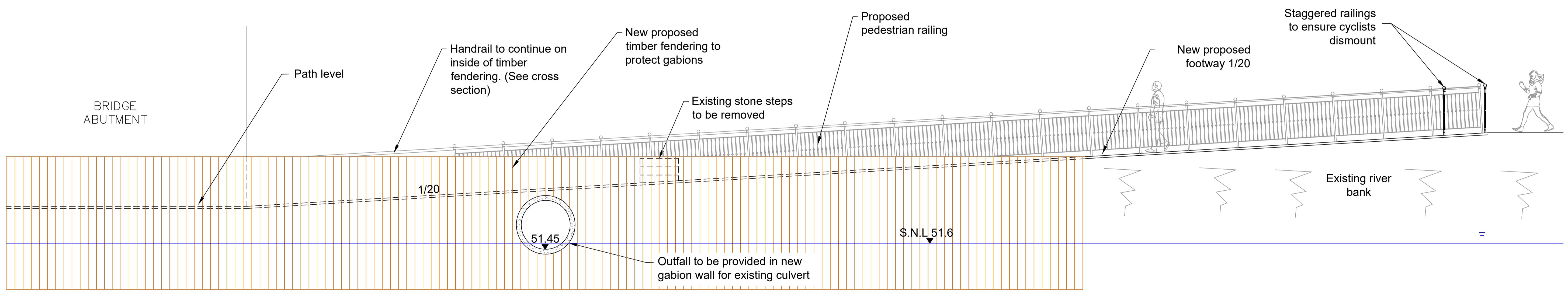
Proposed Elevation Scale 1:50 at A1
