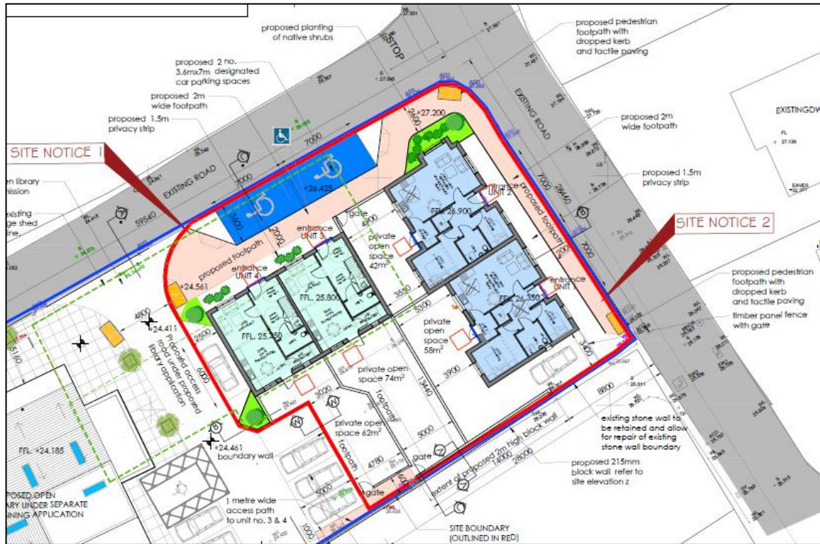
Figure 4– Extract from Planning Drawings (as prepared by Sweeney Architects)
