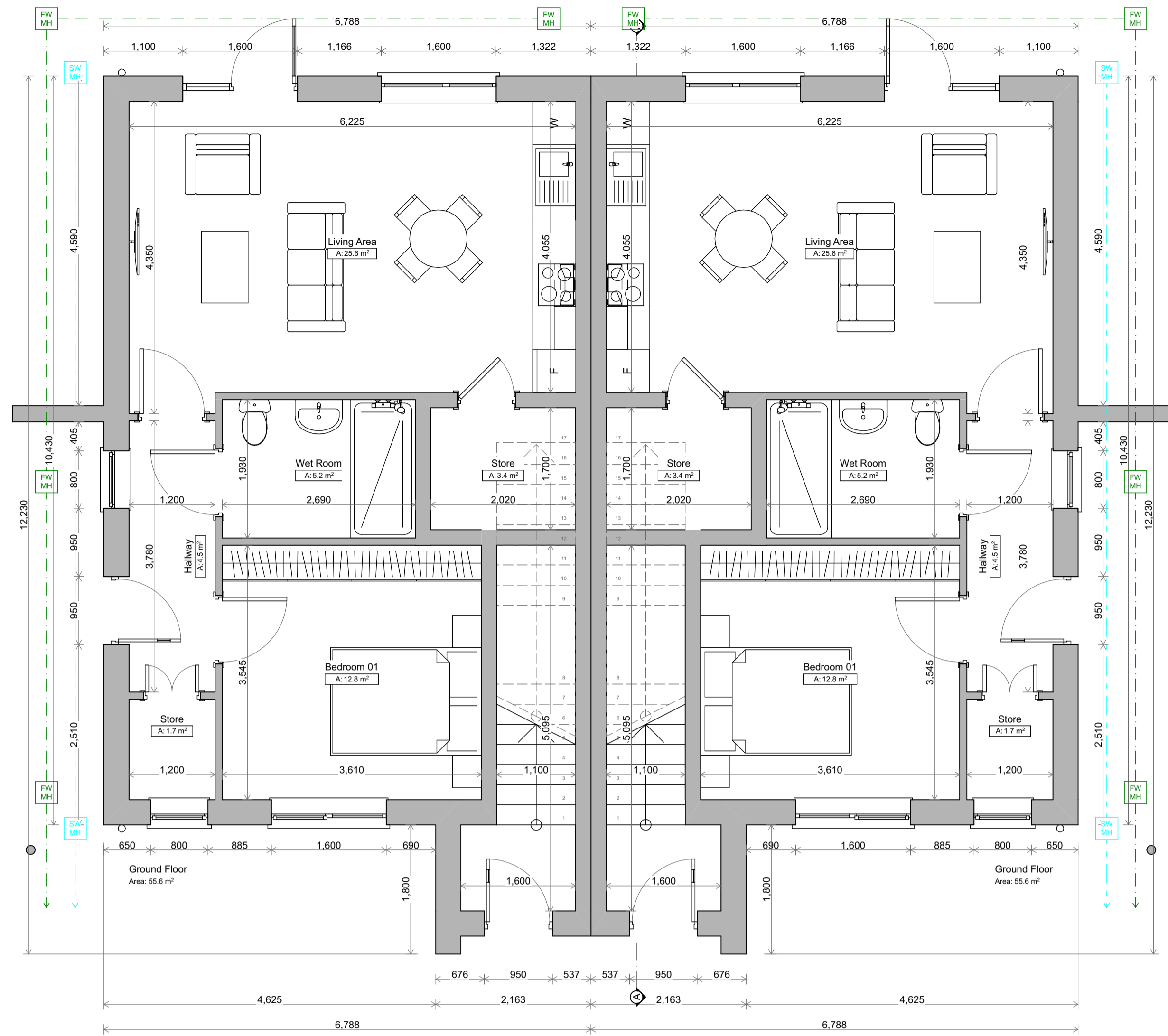
Ground Floor
