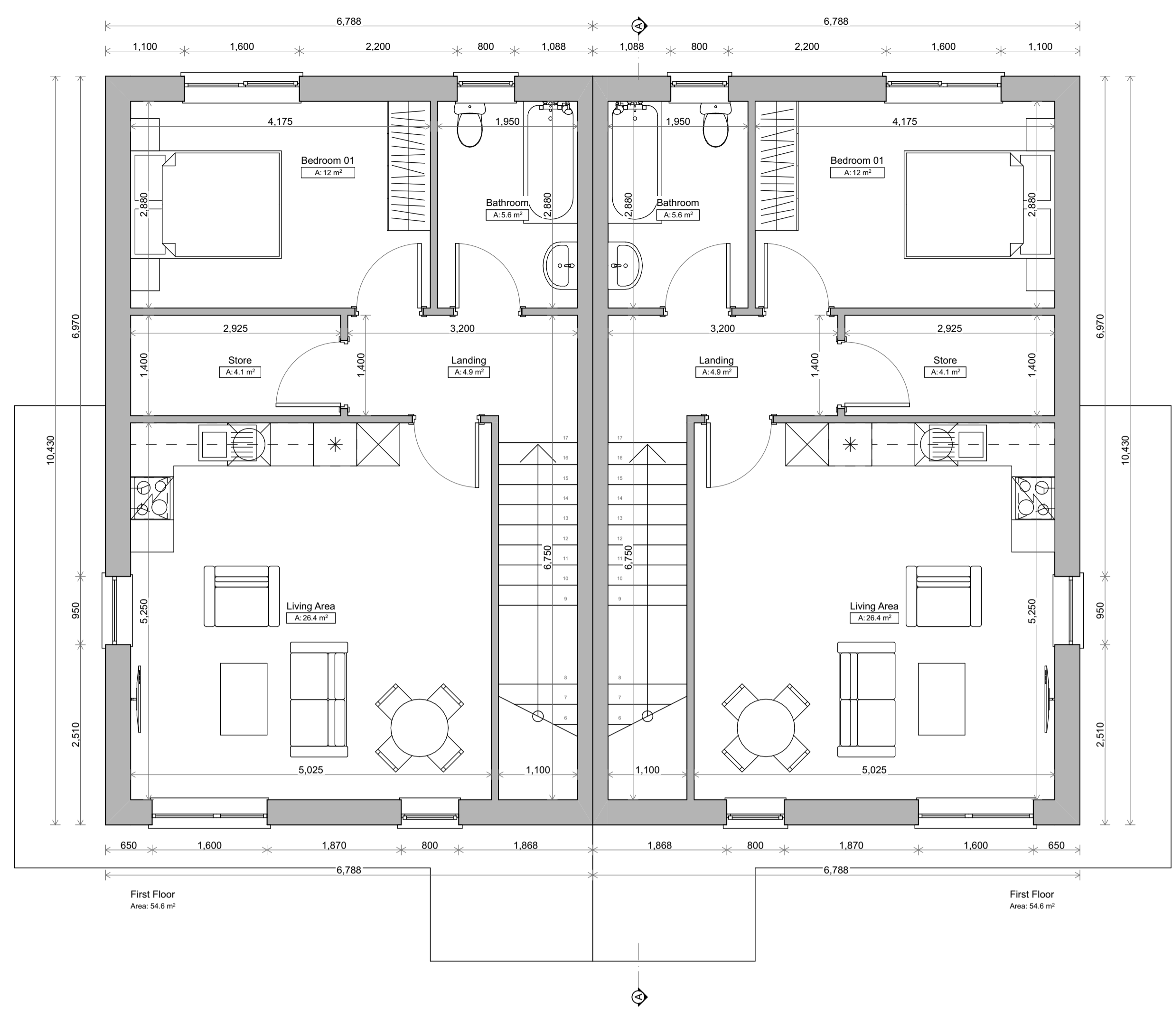
First Floor
