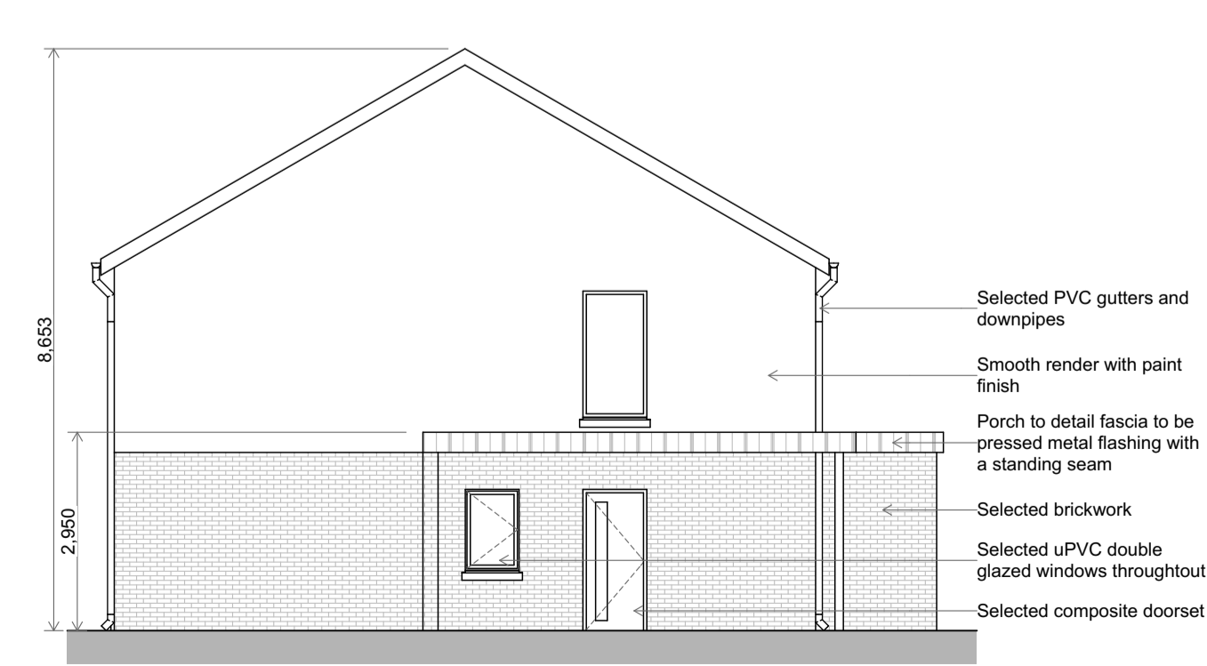
Side Elevation
