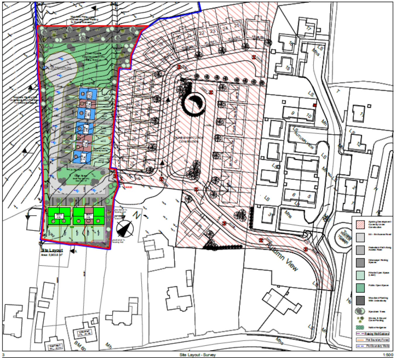
Figure 2 - Site Layout Plan and levels
