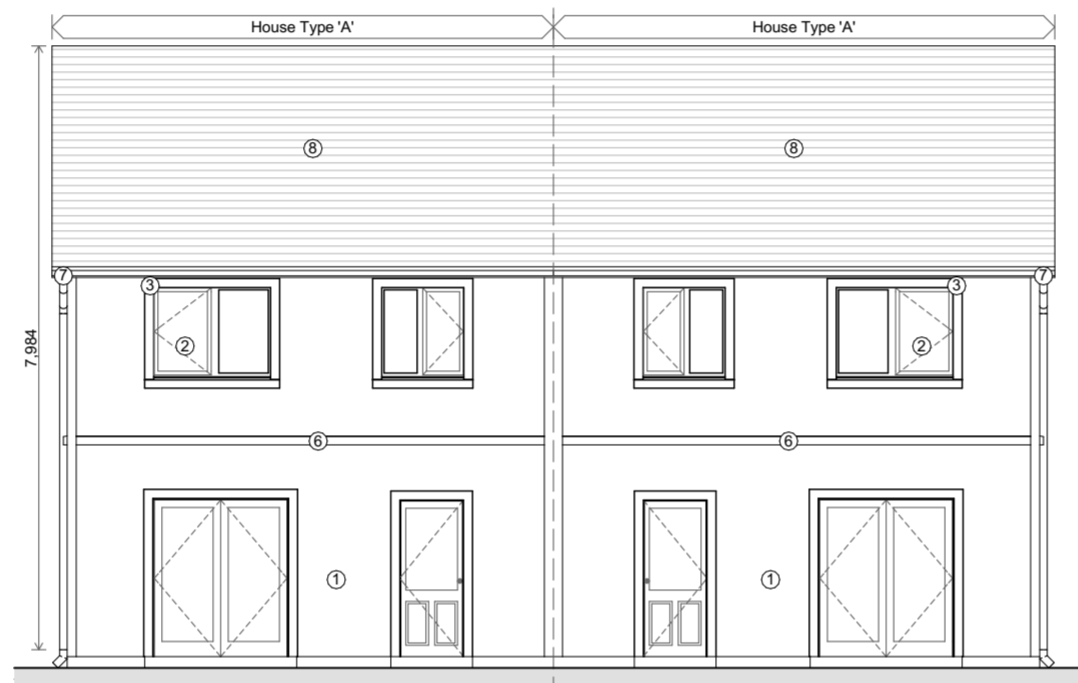
4 Rear Elevation 1:100
