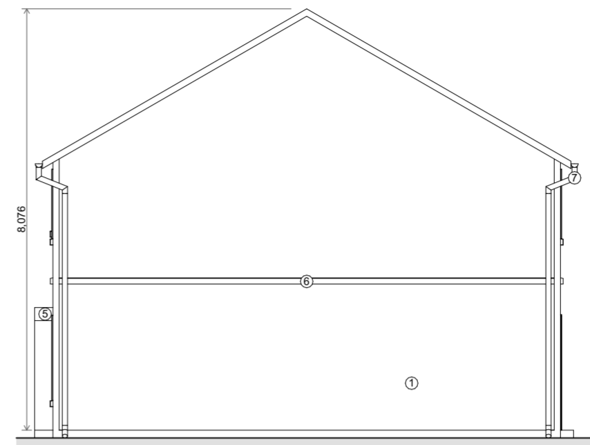
5 Side Elevation 1:100
