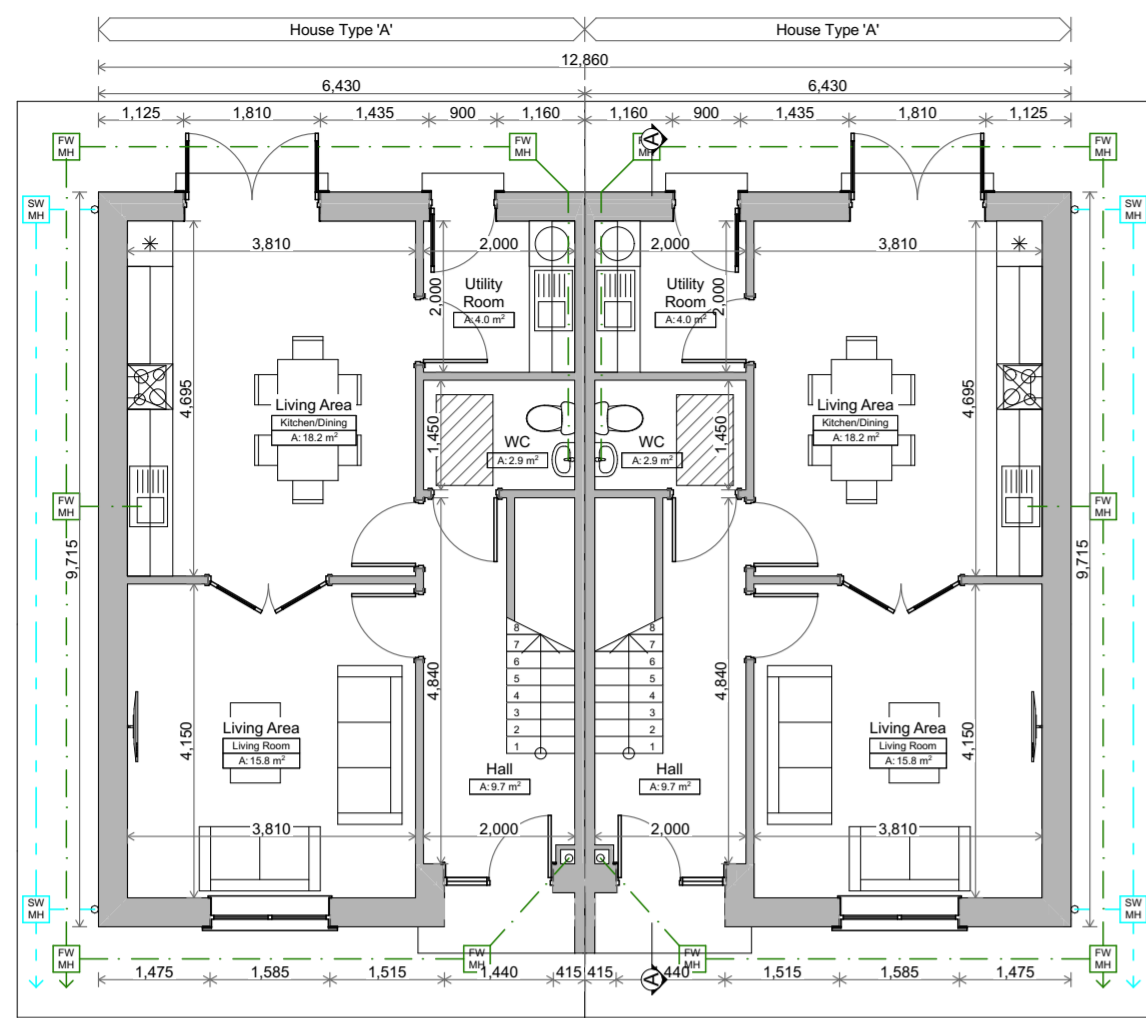
1 Ground Floor Area: 52 m² 1:100
