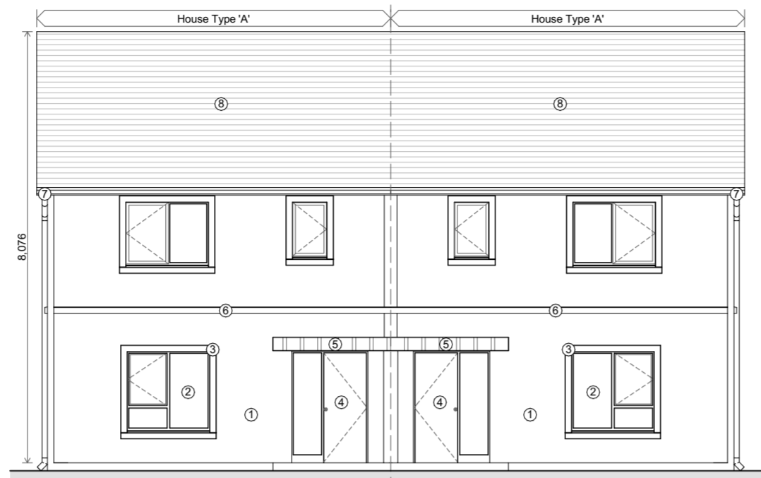
3 Front Elevation 1:100
