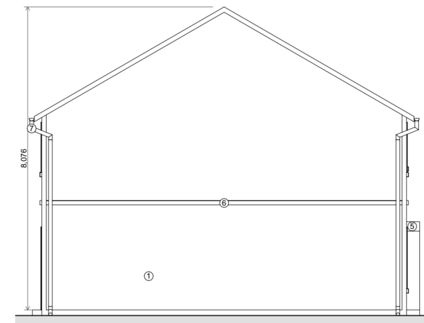
6 Side Elevation 1:100
