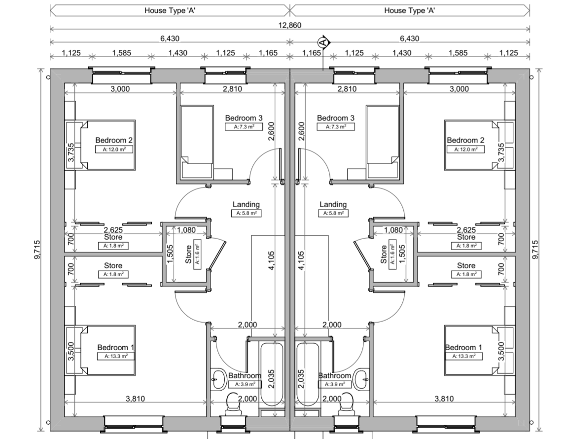
2 First Floor Area: 50.5 m² 1:100
