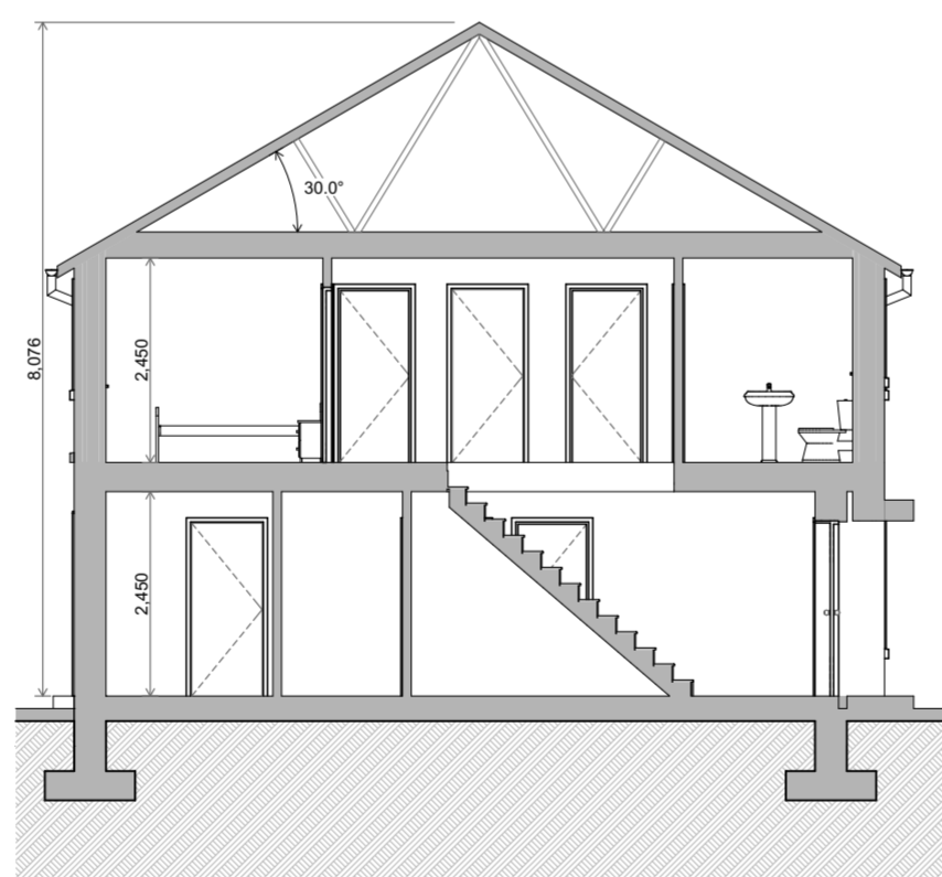
7 Section AA 1:100
