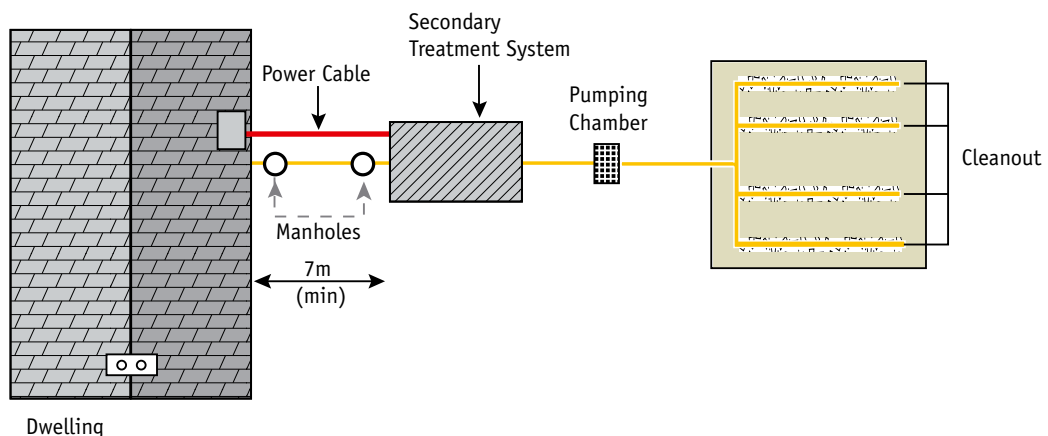
Figure 10.1: Example of a typical low-pressure pipe distribution system
